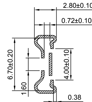
SEC:C-C
