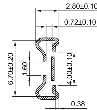
SEC:C-C
