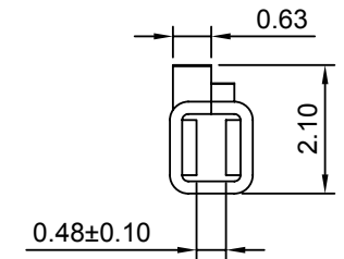
SEC:C-C
