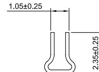
SEC:C-C
