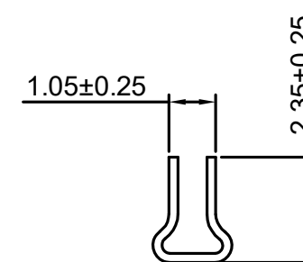
SEC:C-C
