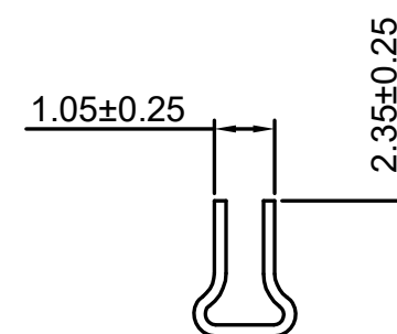
SEC:C-C
