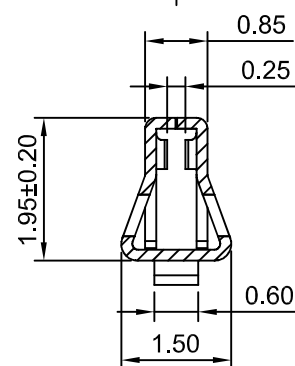
SEC: C-C
