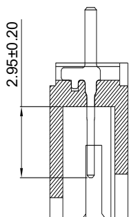
SECTION I-I
