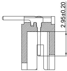
SECTION I-I
