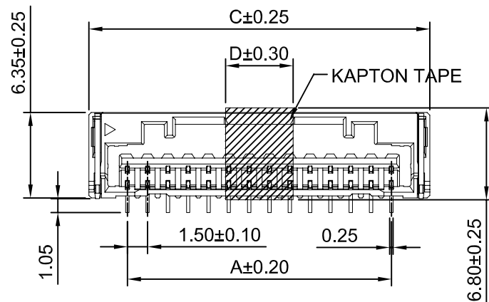
8P~15P KAPTON TAPE FIGURE
