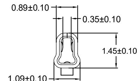
SEC:C-C
