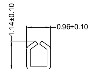
SEC C-C
