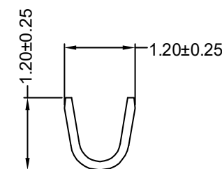
SEC B-B
