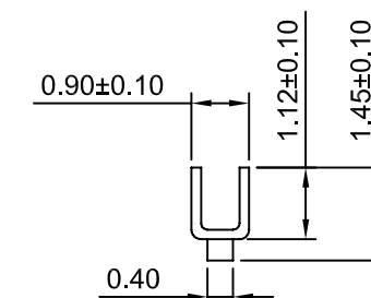
SEC:C-C
