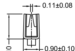
SEC:C-C
