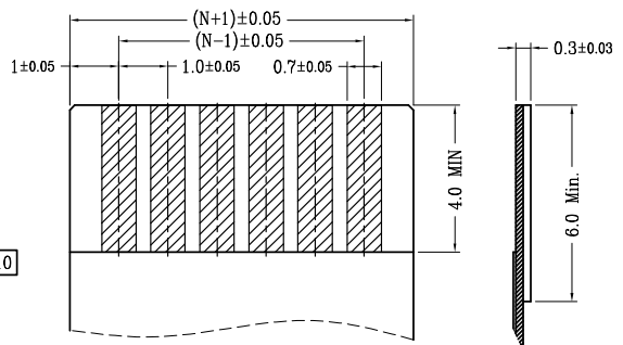
Applicable Flat Cable
