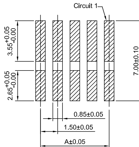
PCB LAYOUT
